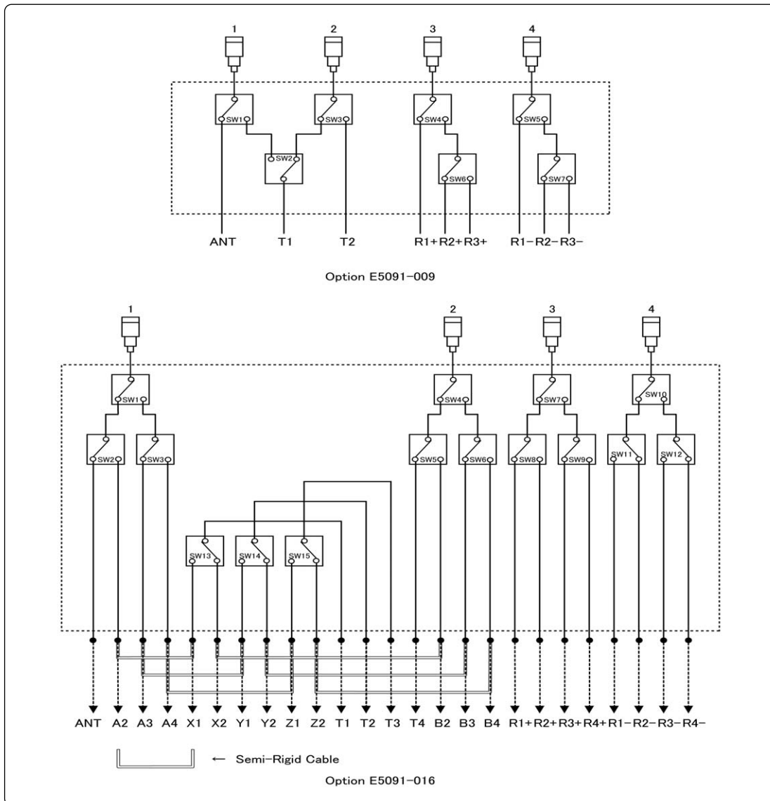
Figure 2-6. Block diagram
